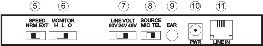
REAR PANEL
